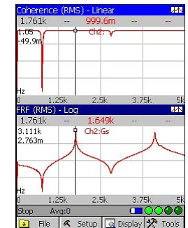
Impact testing
